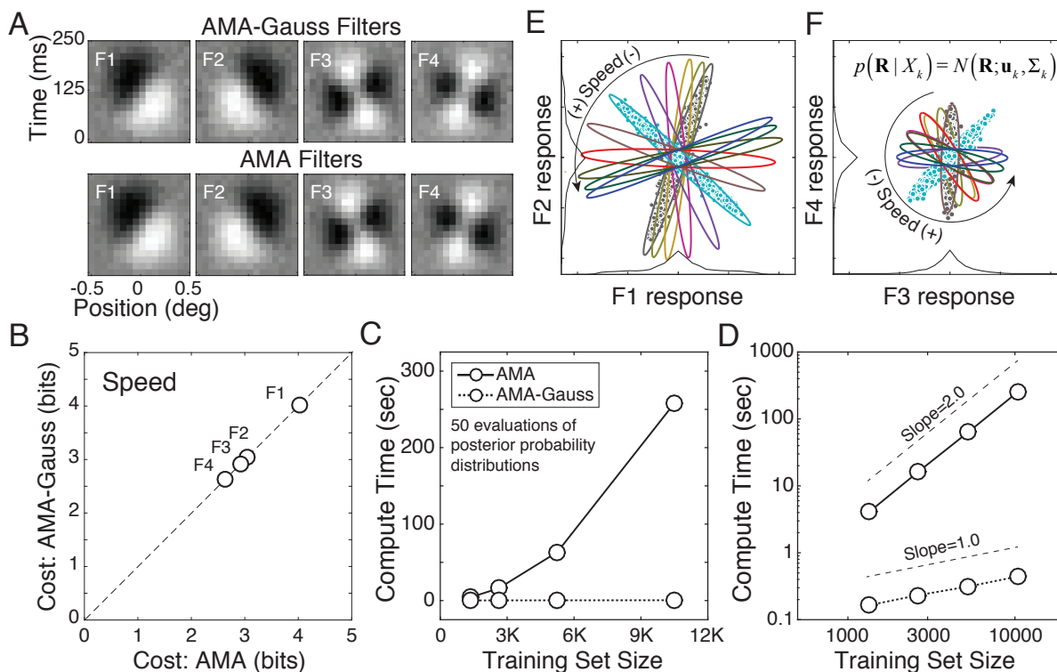
Figure 5: Speed estimation task: filters, cost, compute time, and class-conditional response distributions. A AMA-Gauss and AMA filters for estimating speed ( -8 to +8 deg/sec) from natural image movies are nearly identical; \rho > 0.96 for all filters. B The cost for all the filters for both the models is identical. C Compute time for fifty evaluations of the posterior probability distribution is linear with AMA-Gauss, and quadratic with the full AMA model, in the training set size. D Same data as in C but on log-log axes. E,F Joint filter responses, conditioned on each level of the latent variable, are approximately Gaussian (also see below). Different colors indicate different speeds. Individual symbols represent responses to individual stimuli. Thin black curves show that the filter response distributions, marginalized over the latent variable \mathcal{P}(R) = \sum_{u=1}^{N_{lvl}} \mathcal{P}(R|X_u)\mathcal{P}(X_u) , are heavier-tailed than Gaussians (see Sections 3, 4)
