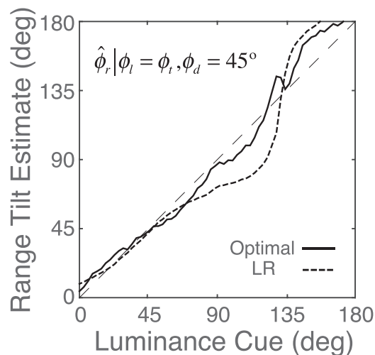
Figure 14. Tilt estimates when the luminance and texture cues are equal and the disparity cue signals a tilt of 45^\circ . If the disparity cue is vetoed (ignored), the estimates should fall on the dashed line. The black curve shows the MMSE optimal estimates, which largely veto disparity when luminance and texture agree. The dashed black curve shows the estimates based on linear cue combination (the LR estimator). For the LR estimator, disparity pulls the estimates in the direction of 45^\circ when luminance/texture cue is in the range of 70^\circ to 130^\circ .
