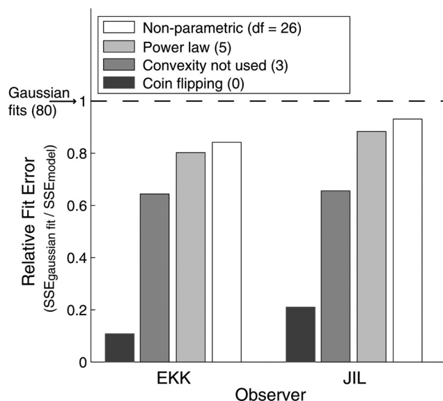
Figure 9. Goodness of fit for four models. The SSE between model predictions and the psychometric data was calculated. Goodness of fit was indexed by SSE_{\text{Gaussian}}/SSE_{\text{model}} so that 1 represents an upper bound. The inverse of those values was then computed and normalized such that 1 represents the normalized inverse error obtained by fitting a cumulative Gaussian to each experimental condition independently (80 free parameters). Larger values represent better fits (lower SSE). Normalized error is shown for four models fit to the data: (1) Coin-flipping model (0 free parameters); (2) a model that assumed that the convexity–depth distributions were the same for convex, concave, and straight-contoured regions; this is equivalent to assuming that convexity was not used when observers estimated perceived depth (3 free parameters); (3) power-law model (5 free parameters); (4) nonparametric model (26 free parameters). We also measured the fits when the difference between the convex and concave distributions was set equal to the difference recovered from the natural-scene statistics. The fits were nearly as poor as the model in which convexity is not used (relative fit error: EKK = 0.62; JIL = 0.67). Finally, we measured the fit errors with Gaussians instead of power laws and found poor fits (relative fit error: EKK = 0.7; JIL = 0.82); JIL’s Gaussian fit is comparable to the power-law fit, but that fit required extremely low-variance disparity likelihoods, which were inconsistent with McKee et al. (1990) and Morgan et al. (2000). We conclude the power-law model is a good description of the internal convexity–depth distributions.
