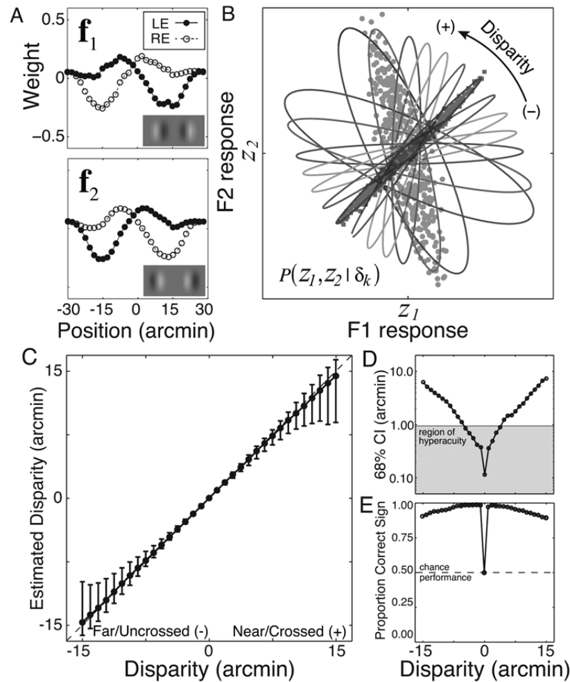
Figure 3. Disparity estimation. A. Two of the eight vertically oriented binocular receptive fields (filters) optimal for disparity estimation. B. Likelihood distributions of first two filter responses for disparities ranging from -15 min to 15 min. Symbols show responses to individual natural image patches for two disparities. Contours indicate 95% of the volume of Gaussian distributions fit to the joint responses. C. Estimation performance on random natural image test patches, for ideal Gaussian mixture model (GMM) using all eight optimal filter responses. Symbols are mean estimates and error bars represent 68% confidence intervals. D. Confidence intervals of estimates as
